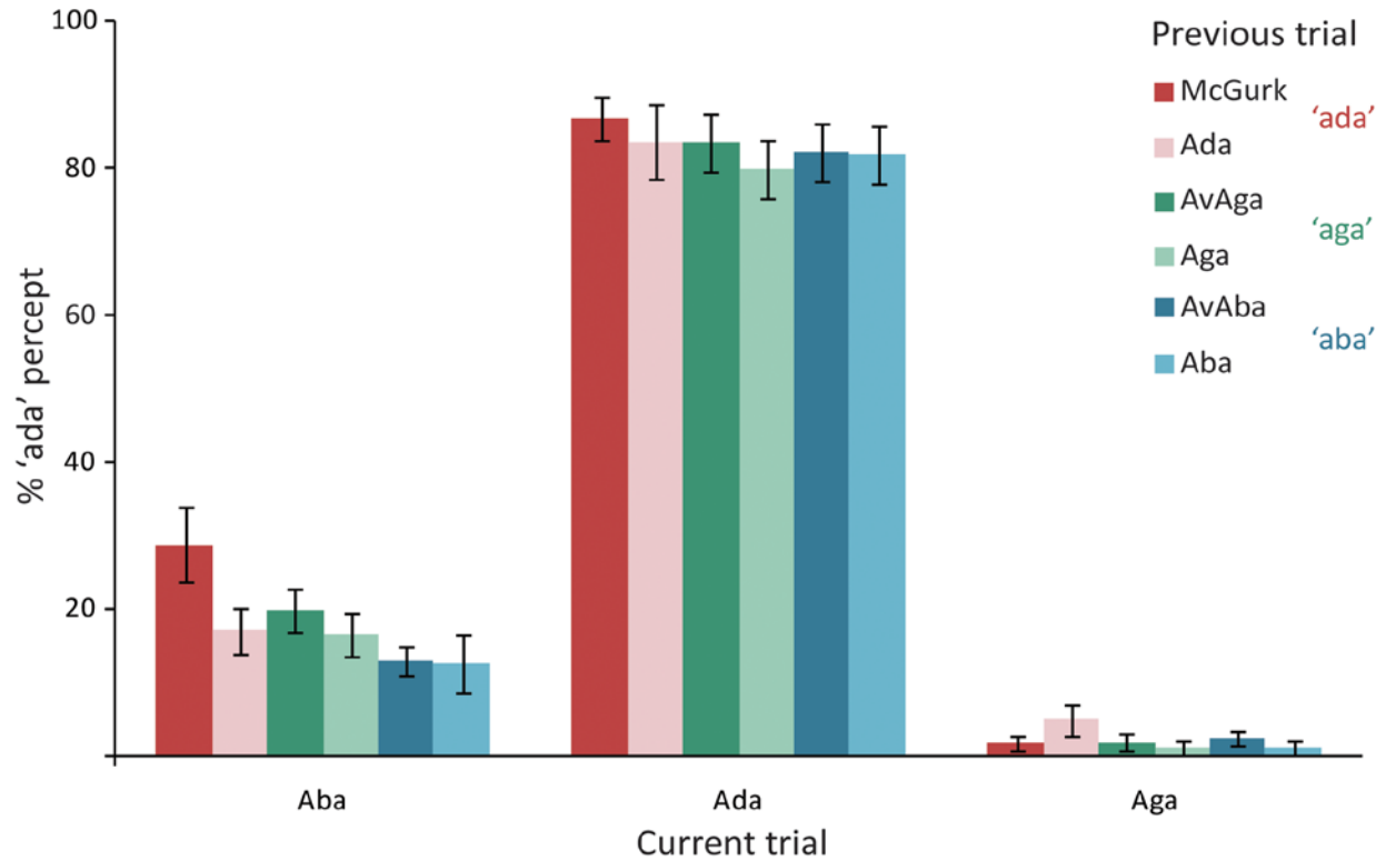
Supplementary Figure S1. The proportion of 'ada' percepts on all auditory trials sorted according to their previous trial. The preceding trial was audiovisual (dark; McGurk, AvAga, AvAba) or auditory (light; Aba, Ada, Aga) and could be perceived as 'ada' (red), 'aga' (green) or 'aba' (blue). Error bars display standard error of the mean.
